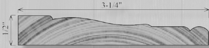
WC226 1/2" x 3-1/4"
