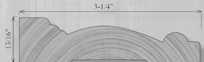
C3230/WC271 13/16" x 3-1/4"
