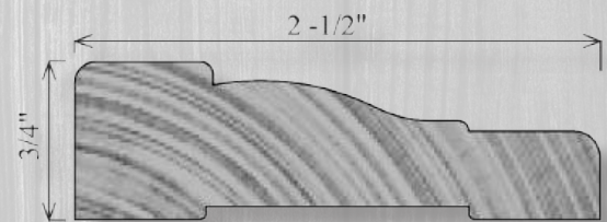
WC282 3/4" x 2-1/2"
