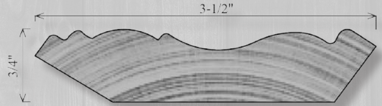
WCR44B 3/4" x 3-1/2"
