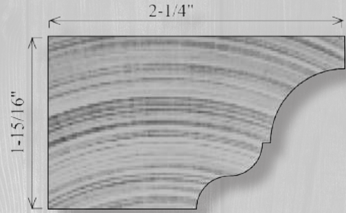
CN227 1-5/16" x 2-1/4"
