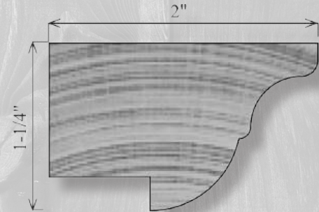
CN200 1-1/4" x 2"
