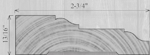
C275 13/16" x 2-3/4"
