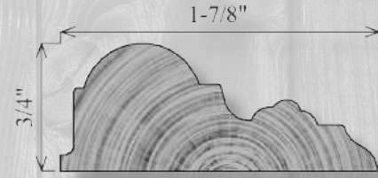
CR189 3/4" x 1-7/8"
