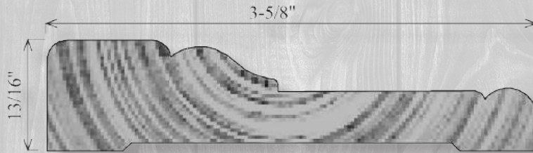
C356 13/16" x 3-5/8"
