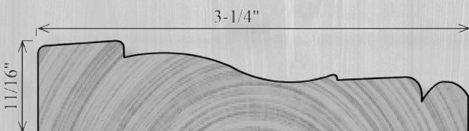
C3270/WC254 11/16" x 3-1/4"
