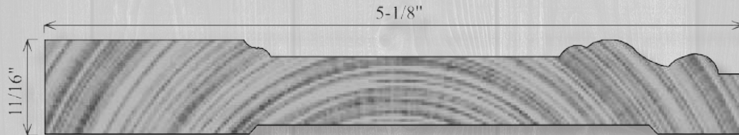
B512 11/16" x 5-1/8"
