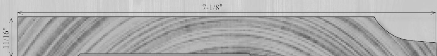
B712 11/16" x 7-1/8"
