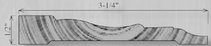
C324 1/2" x 3-1/4"
