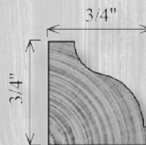
CV075 3/4" x 3/4"
