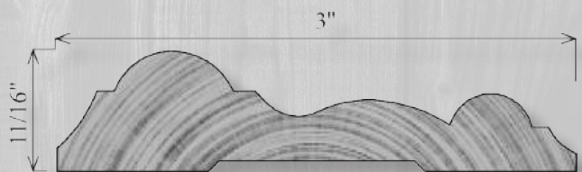
CR300/WCH73B 11/16" x 3"
