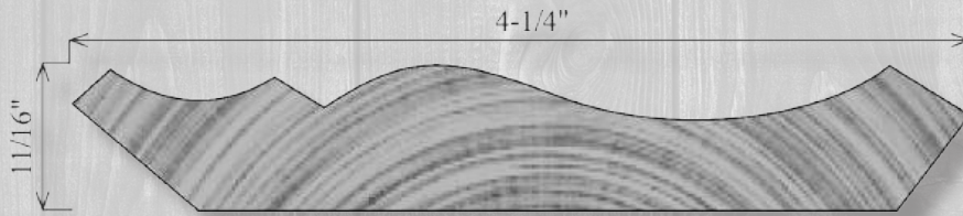
CN4250 11/16" x 4-1/4"
