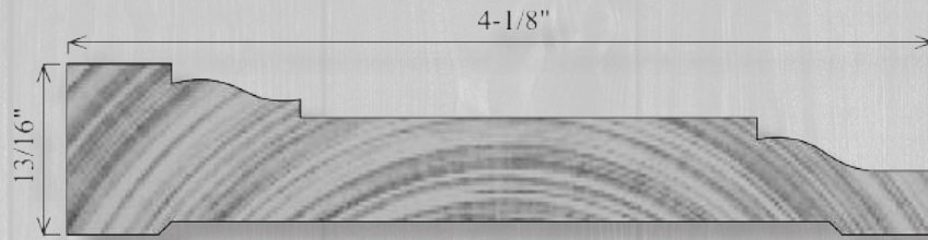
C413 13/16" x 4-1/8"
