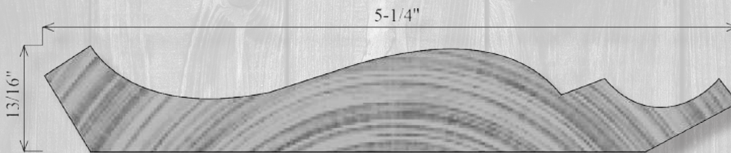
CN5250 13/16" x 5-1/4"
