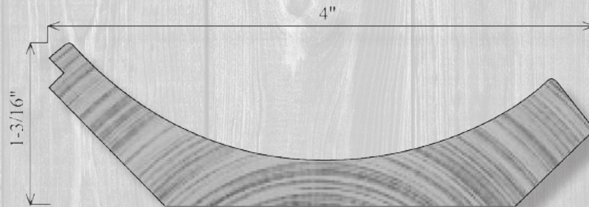
CN400 1-3/16" x 4"
