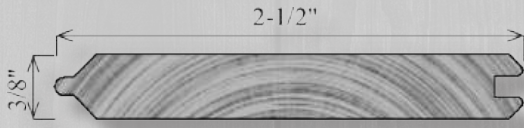
PG250 — 3/8" x 2-1/2" PG326 — 3/8" x 3-1/4"
