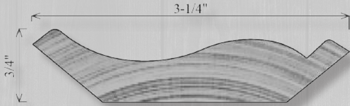
WCR44A 3/4" x 3-1/4"
