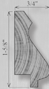
BC162/ WBC11 3/4" x 1-5/8"
