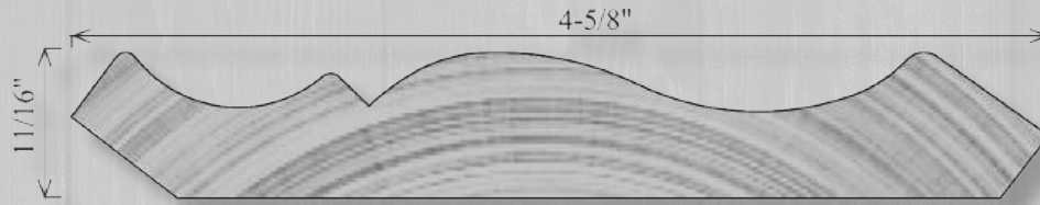
WCR43A 11/16" x 4-5/8"
