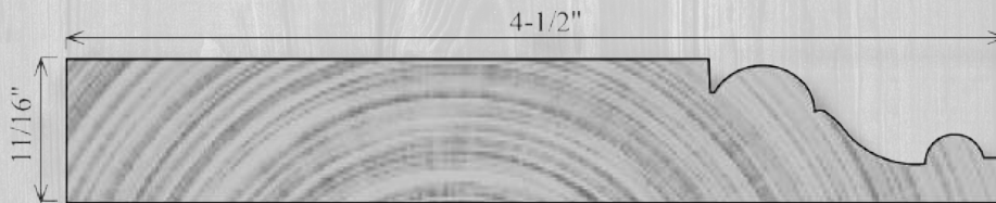
WB151 11/16" x 4-1/2"
