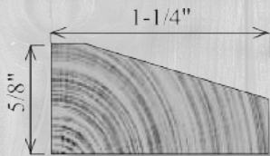
SP1625 5/8" x 1-1/4"
