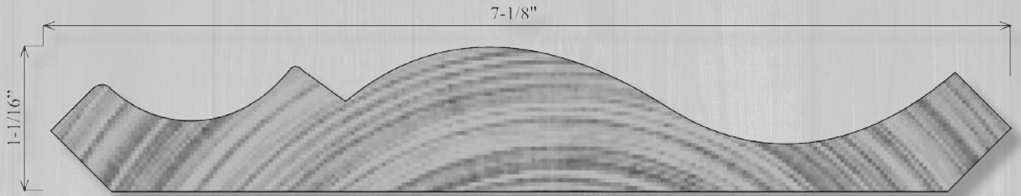
CN706 1-1/16" x 7-1/8"
