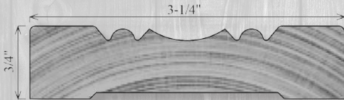
C318 3/4" x 3-1/4"
