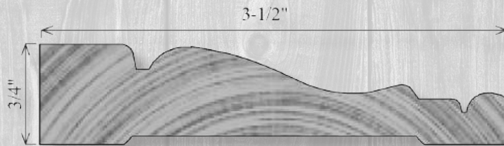
C350 3/4" x 3-1/2"
