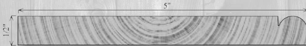
WB123 1/2" x 5"
