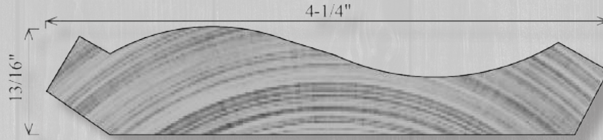
WCR45 13/16" x 4-1/4"
