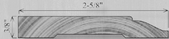
B262 – 3/8" x 2-5/8"
