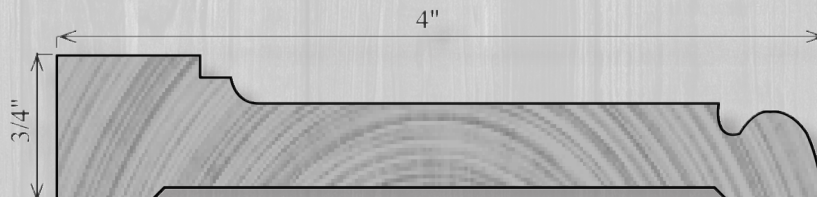
C402 3/4" x 4"
