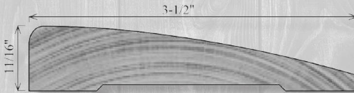
WC257A 11/16" x 3-1/2"
