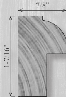
BB143 1-7/16" x 7/8"
