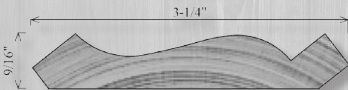
WCR41A 9/16" x 3-1/4"
