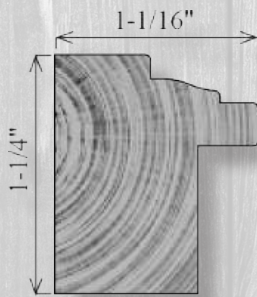
BB1240 1-1/4" x 1-1/16"
