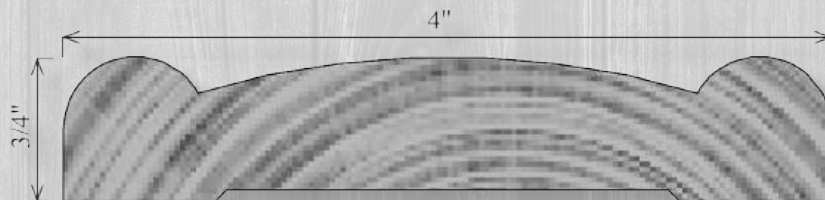
C400 3/4" x 4"
