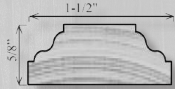
CR150 5/8" x 1-1/2"
