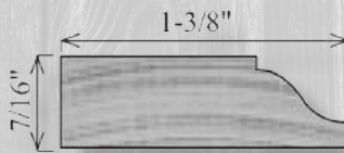
WST74 7/16" x 1-3/8"
