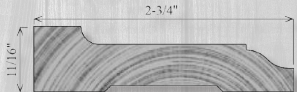
C277 11/16" x 2-3/4"
