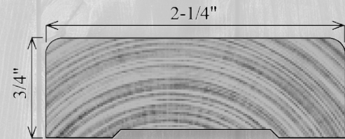
C223 - 3/4" x 2-1/4" C331 - 3/4" x 3-1/4"
