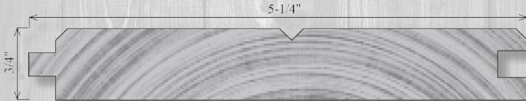
PG526 3/4" x 5-1/4"
