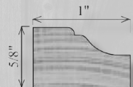
WGB51 5/8" x 1"
