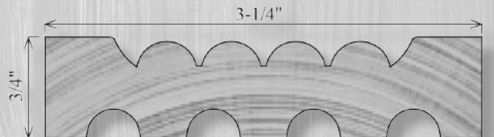
WC264F 3/4" x 3-1/4"
