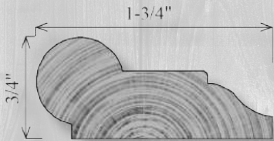
CR175 3/4" x 1-3/4"
