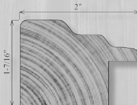
BB200 1-7/16" x 2"
