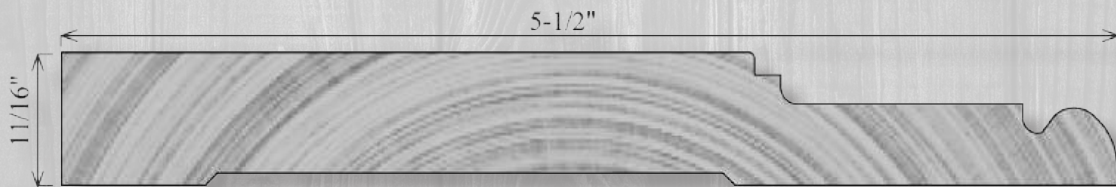
B551 11/16" x 5-1/2"
