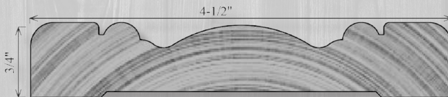
C450 13/16" x 4-1/2"
