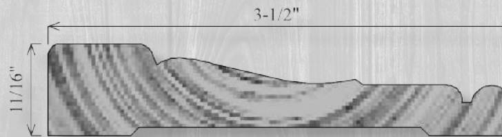
C352 11/16" x 3-1/2"
