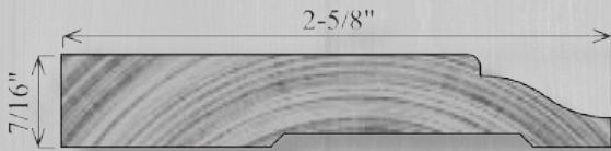
B261 – 7/16" x 2-5/8"
