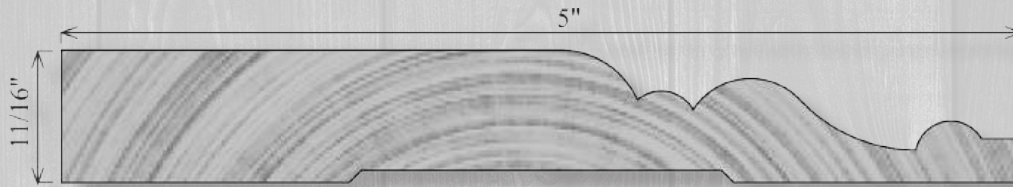
B487 11/16" x 5"
