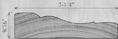
WC230 9/16" x 2-1/4"
