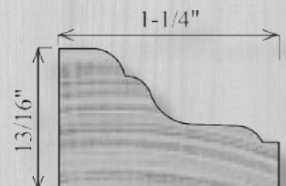
CV126 13/16" x 1-1/4"
