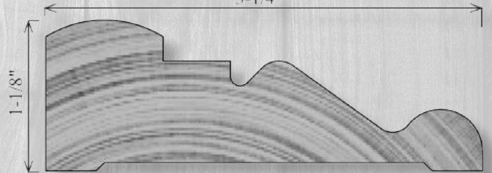
C319 1-1/8" x 3-1/4"
