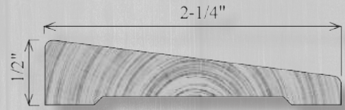
C2252/WC223A 1/2" x 2-1/4"
