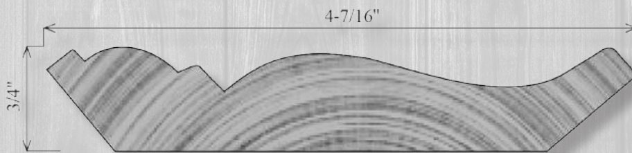
CN444 3/4" x 4-7/16"
