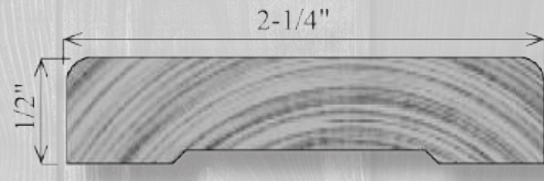
C2240 - 1/2" x 2-1/4" C3300 - 1/2" x 3-1/4"
