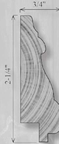
BC225 3/4" x 2-1/4"
