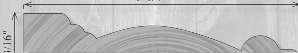
B531 5/8" x 5-1/4"
