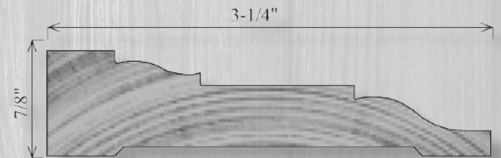
C321 3/4" x 3-1/4"
