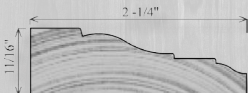
WC241 11/16" x 2-1/4"
