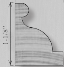
PM112 7/8" x 1-1/8"
