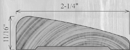
C228 11/16" x 2-1/4"
